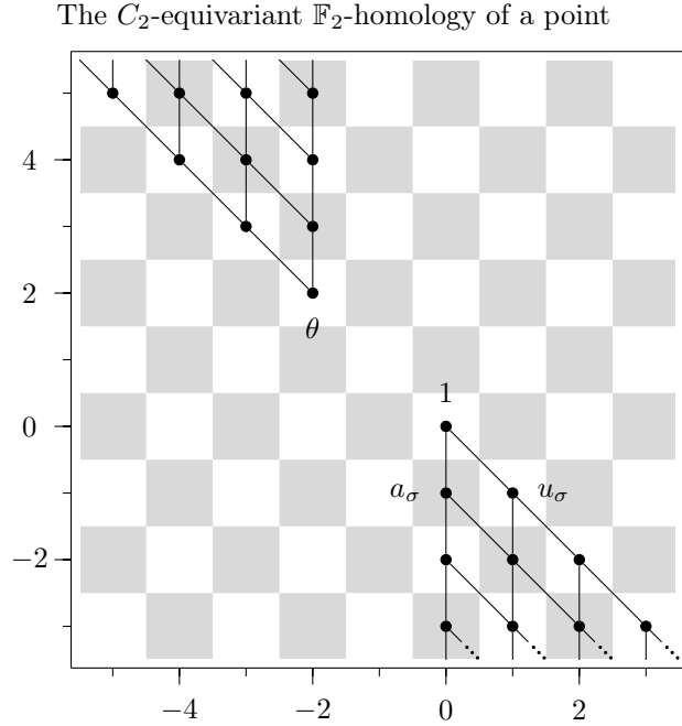
FIGURE 1. The bigraded homotopy groups of \mathbb{F}_2 depicted on a (p, q) coordinate system. Vertical lines going down denote multiplication by a_\sigma . Diagonal lines going down-right denote multiplication by u_\sigma .
