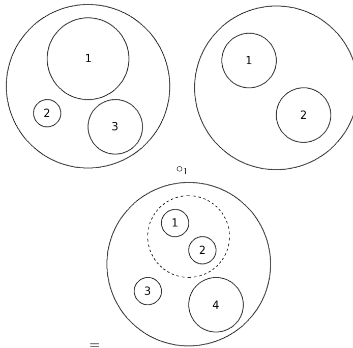
FIGURE 3. Example of partial composition in the little discs operad
