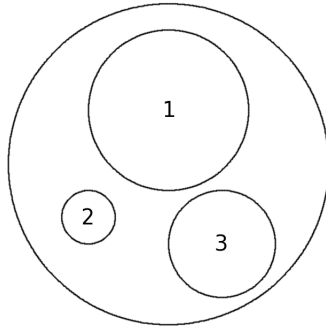
FIGURE 2. Little discs configuration in D^2(3)
