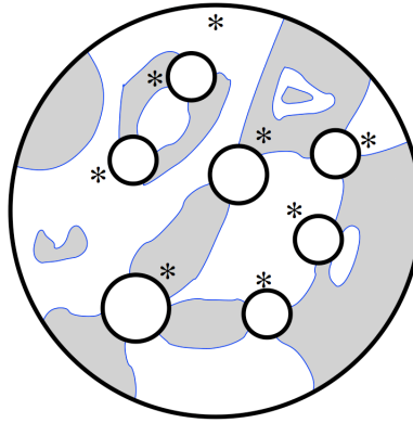
FIGURE 4. A Tangle (Courtesy of V.F.R. Jones)
